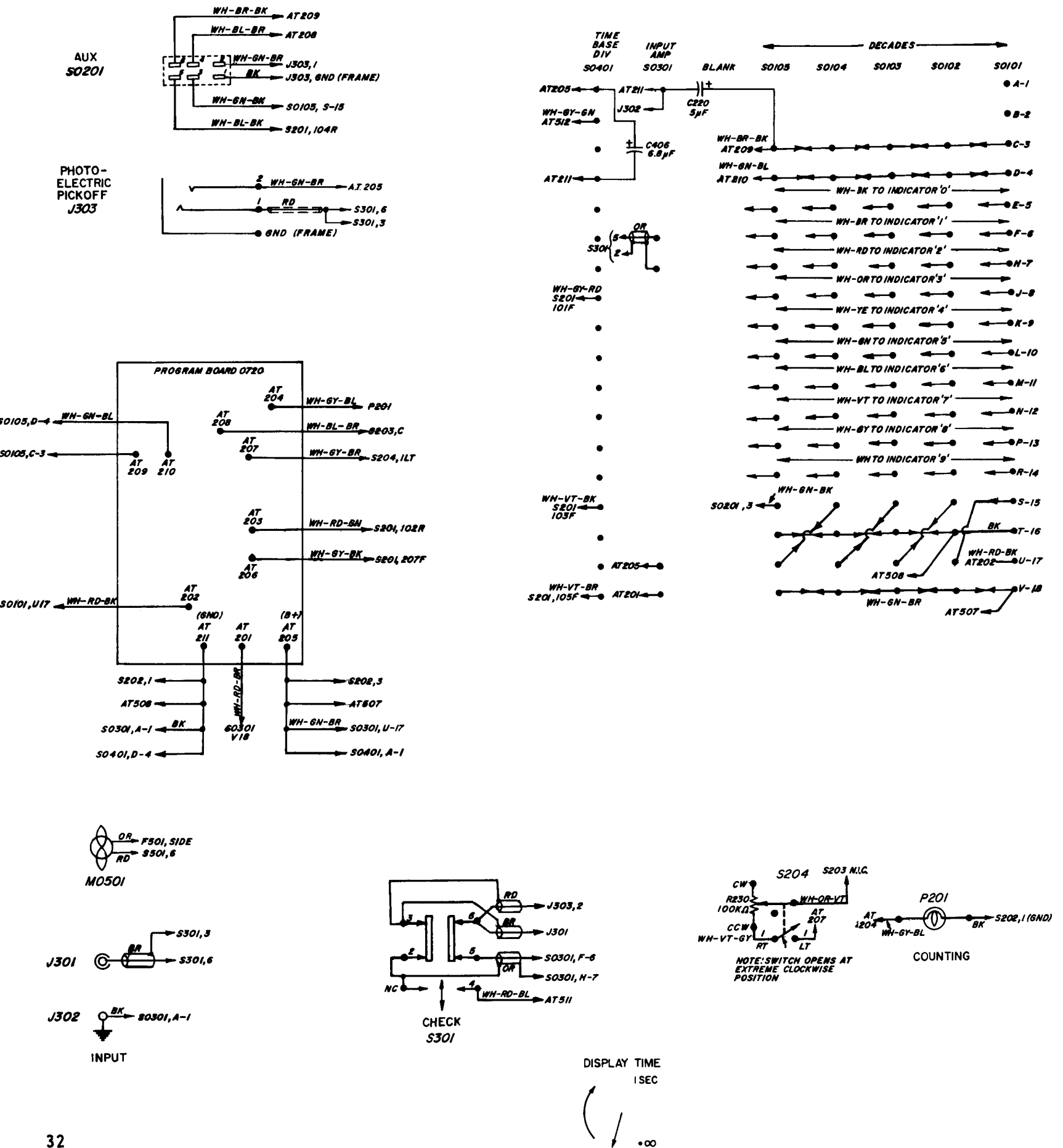
Figure 4-16. Interconnection
