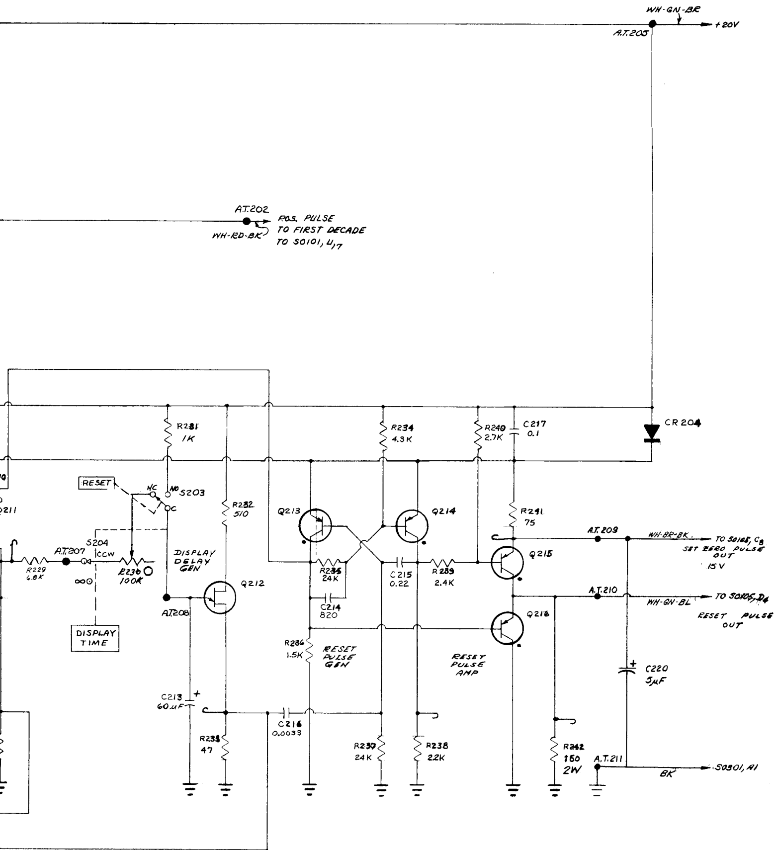
the program control circuit.
