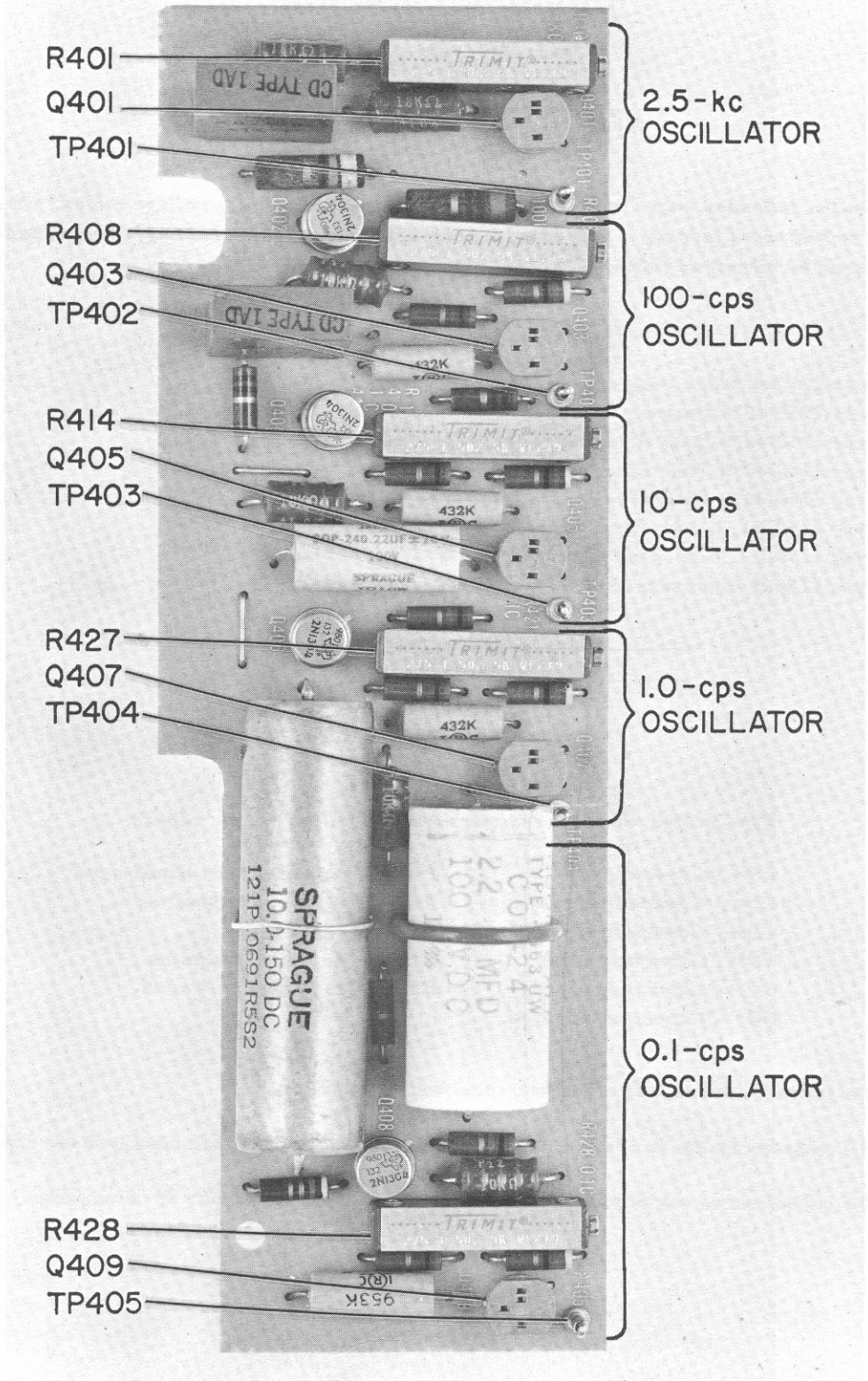
Figure 4-1. Time-base divider etched board used in the Digital Frequency Meter.
