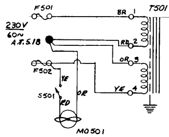
POWER TRANSFORMER (T501) PRIMARY CONNECTIONS FOR 115 OR 230 VOLT LINE
