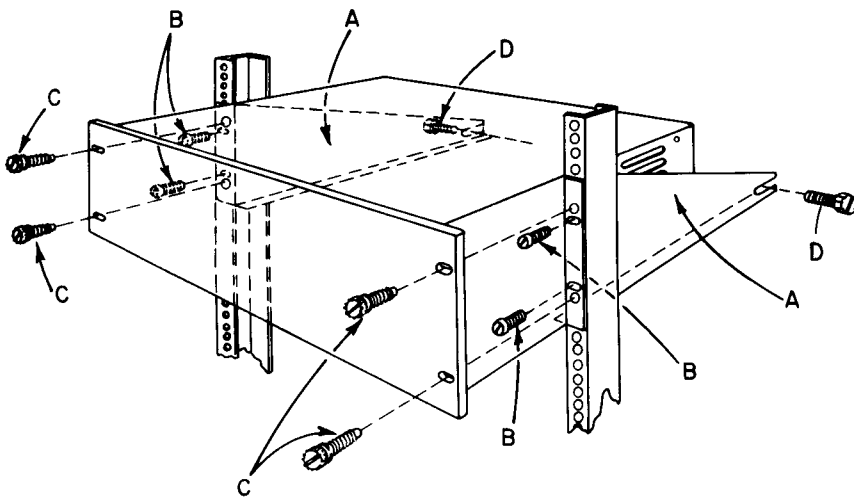
Figure 2-1. Installation of relay-rack model, Type 1150-AR.
