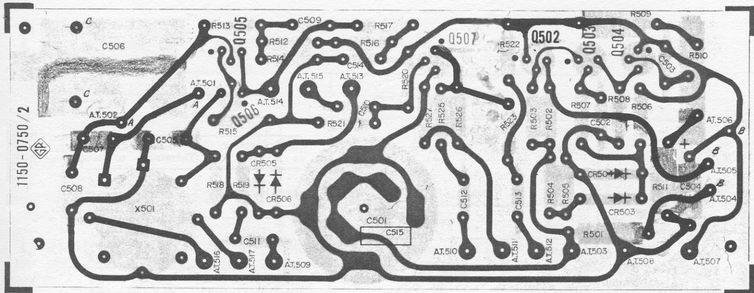
Figure 4-11. Power supply and oscillator etched board.
