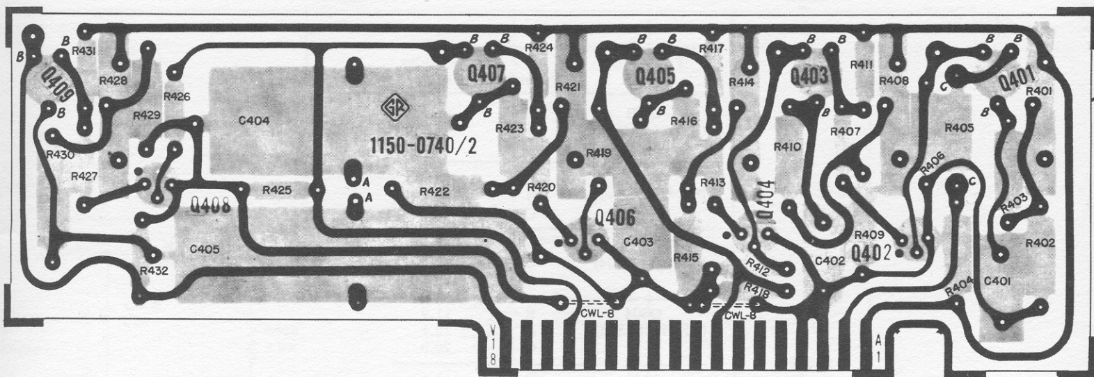
Figure 4-9. Time-base divider etched board.
